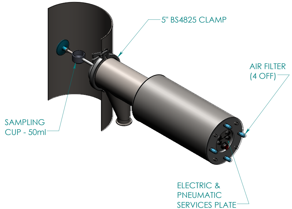
ISOMETRIC VIEWS
