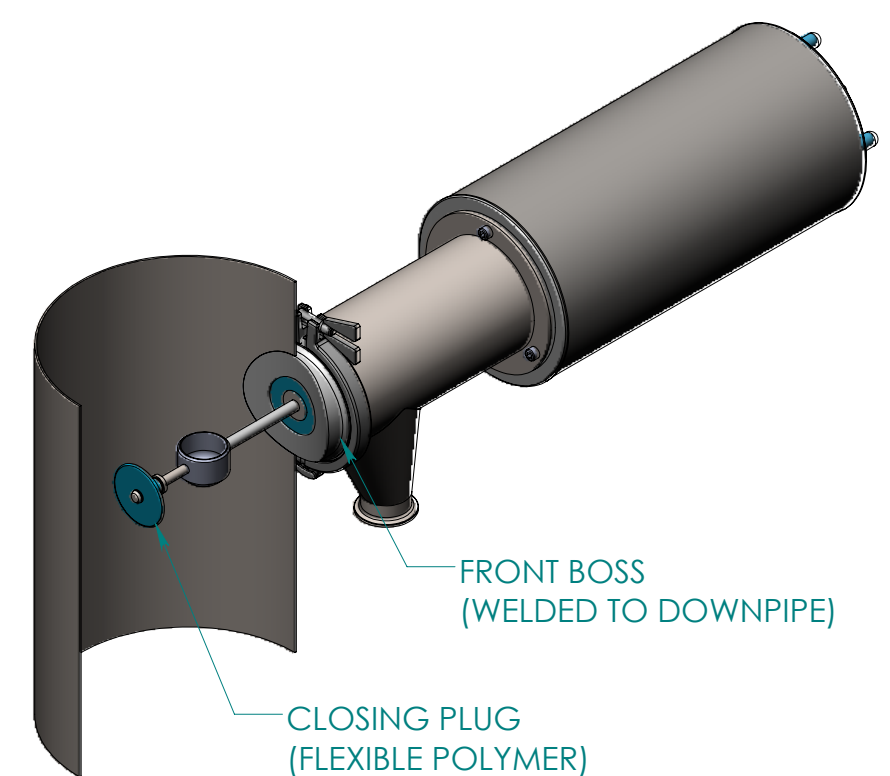
ISOMETRIC VIEWS
