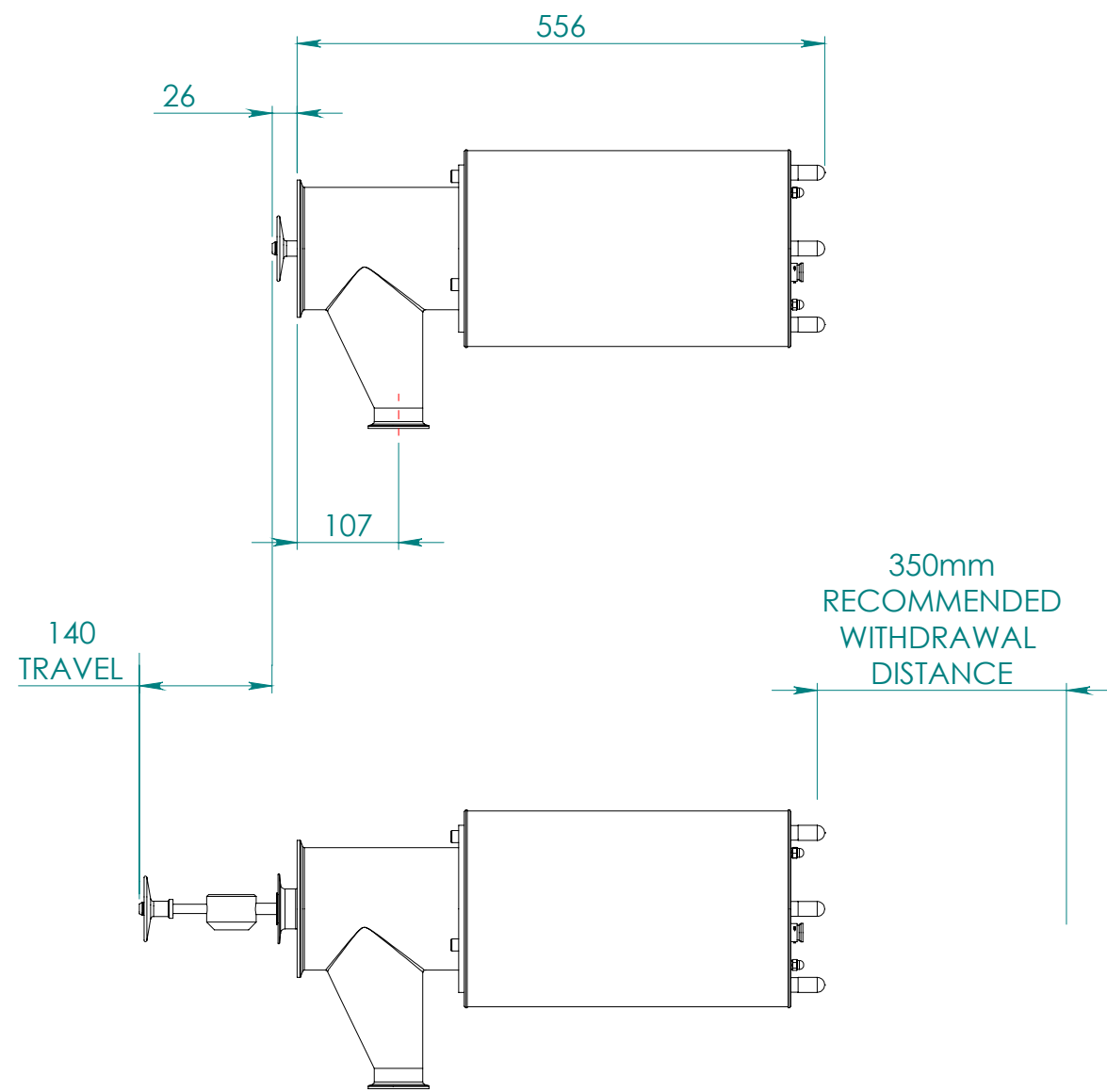
SIDE VIEW UNIT WITH SHAFT IN EXTENDED POSITION
