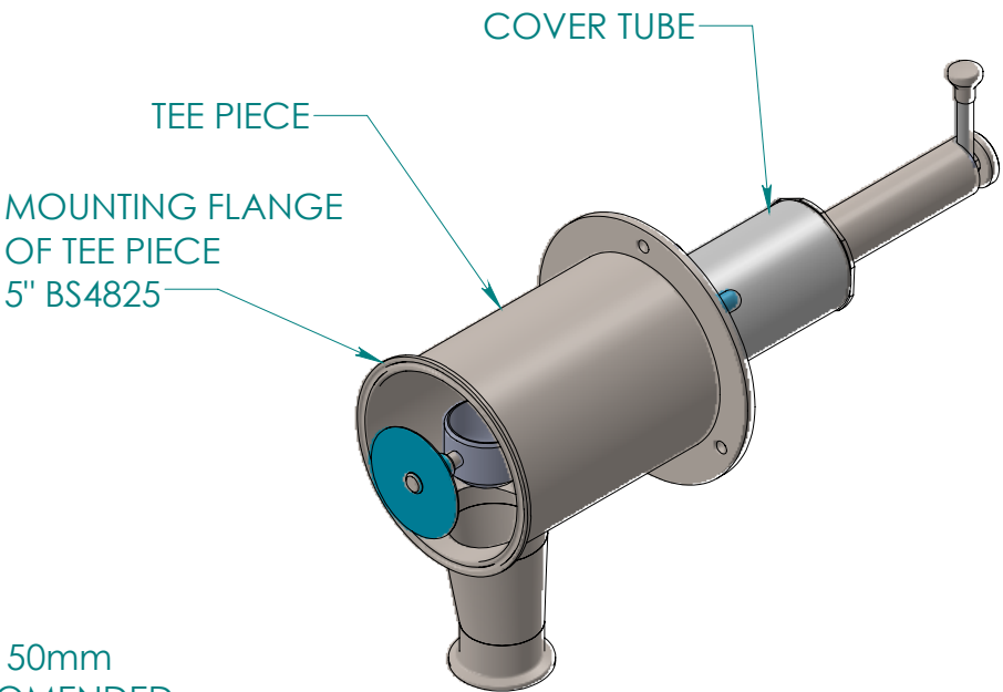
ISOMETRIC VIEW
